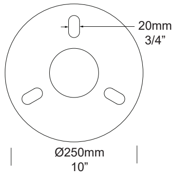
Flange Mount
