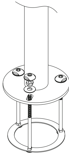
Flange Mount
